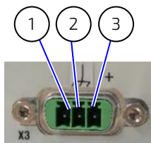
Figure 20: Input Power Connector
