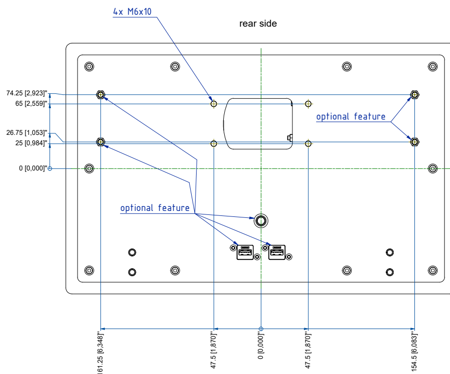
Rear View
