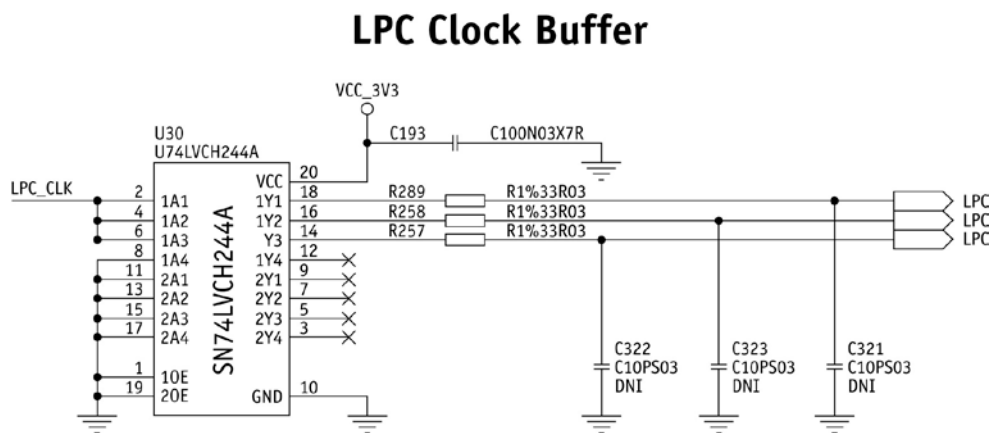
Figure 7: LPC Clock Buffer
