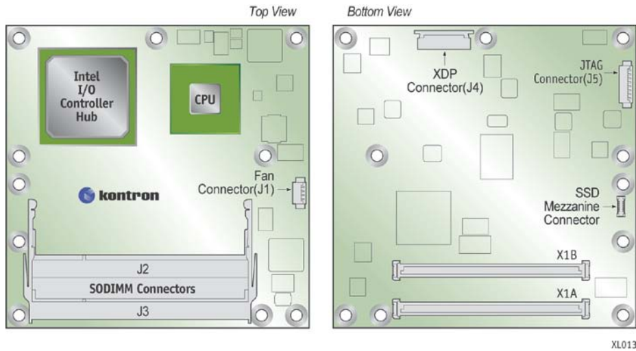
Figure 4: Onboard Connectors
