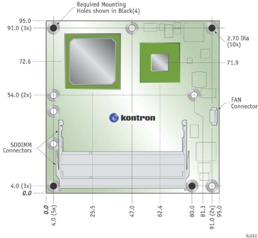
Figure 2: microETXexpress®-PV-XT COM Mechanical Drawing
